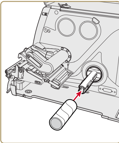
Route the Liner Around a Cardboard Core
