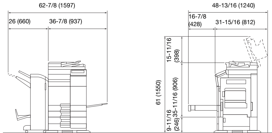
ineo 224e/284e/364e + DF-624 + PC-210 + FS-534 + SD-511
